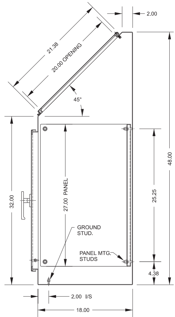
Section Y-Y
